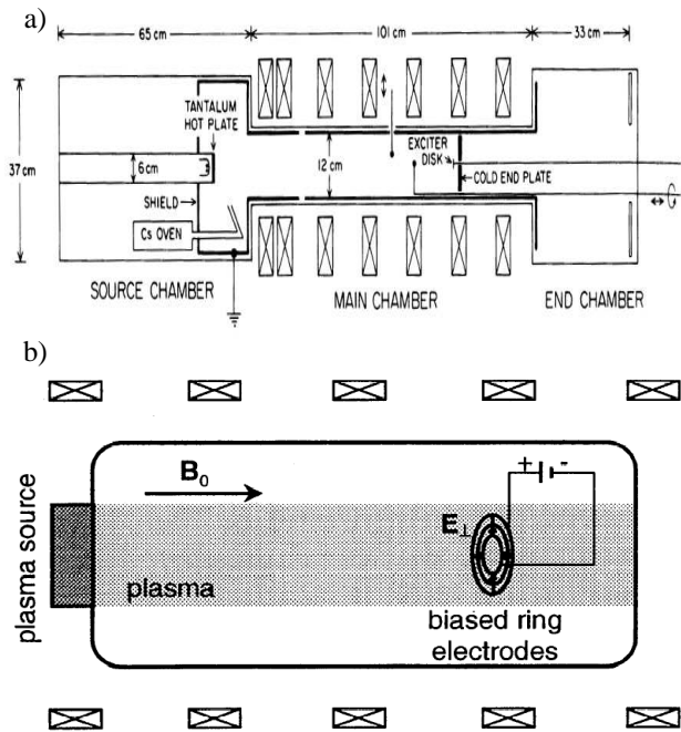
FIG. 1: Typical setup for studying Electrostatic Ion Cyclotron (EIC) wave. a) Used by Motley and D'Angelo [18] to excite current driven EIC. The picture is taken from Ref. [19]. b) Used by Koepke et al. to excite inhomogeneous energy density driven EIC. The picture is taken from Ref. [20].
