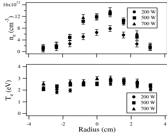
FIG. 5: Plasma density and electron temperature for various rf power to the saddle antenna. As rf power is raised above 500 W the high plasma density helicon discharge is observed. B=782 Gauss, P=1\text{mTorr} .
