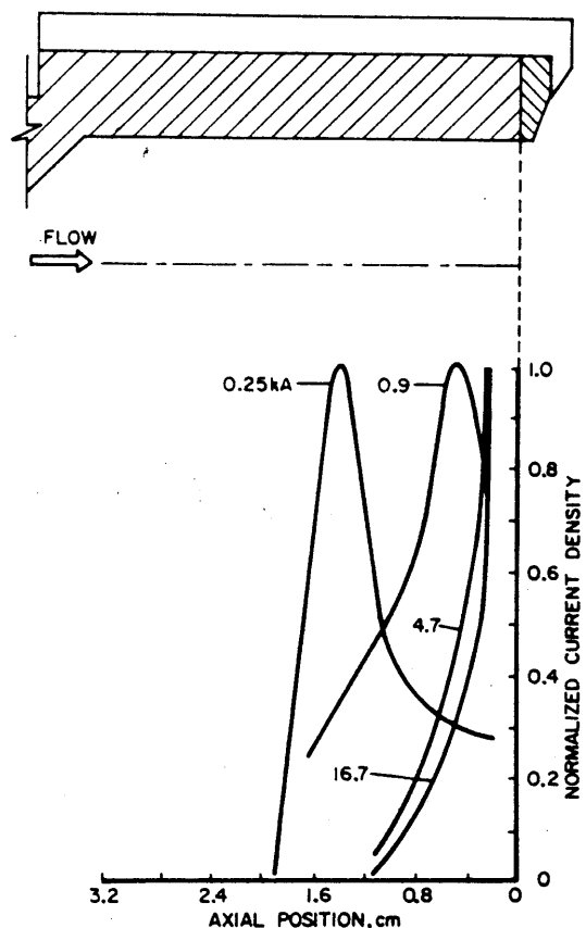
Fig. 6 Current density distributions, 0.2 g/sec.
