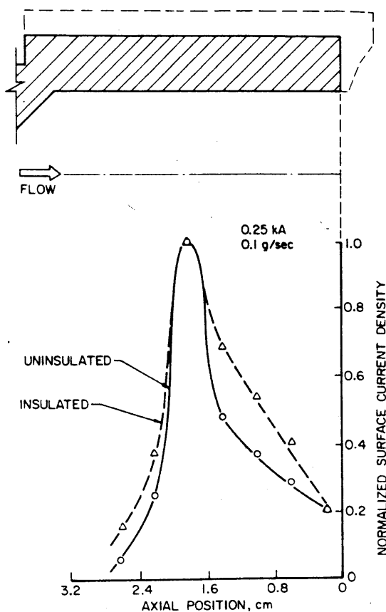
Fig. 9 Current density distributions.
