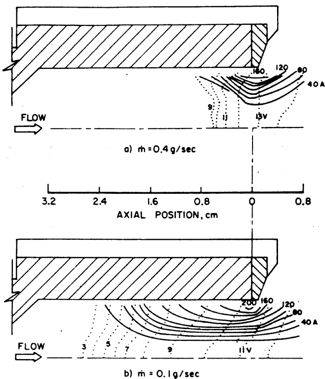
Fig. 7 Enclosed current and potential profiles, 0.25 kA.
