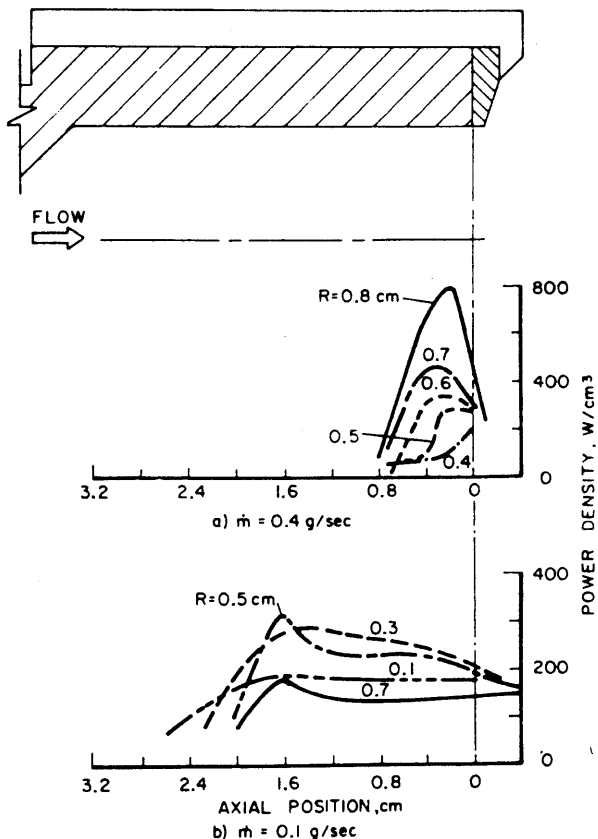
Fig. 8 Power density profiles, 0.25 kA.
