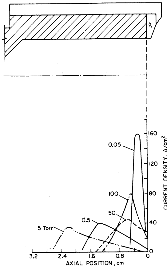
Fig. 10 Current density profiles; J = 0.25 kA, no flow.
