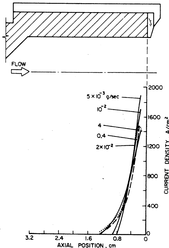
Fig. 5 Current density profiles, 4.7 kA.
