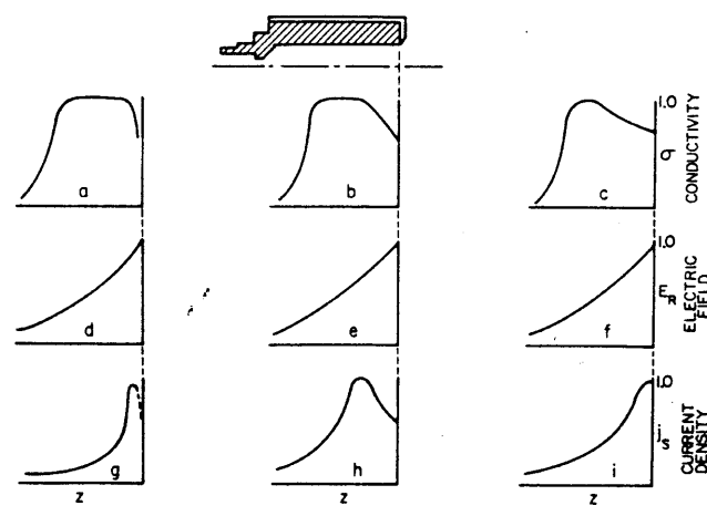
Fig. 12 Surface conductivity, electric field, and current density profiles (schematic).
