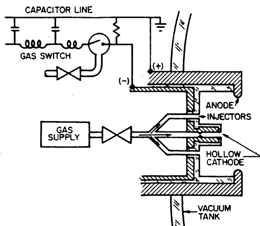
Fig. 1 Hollow cathode facility.
