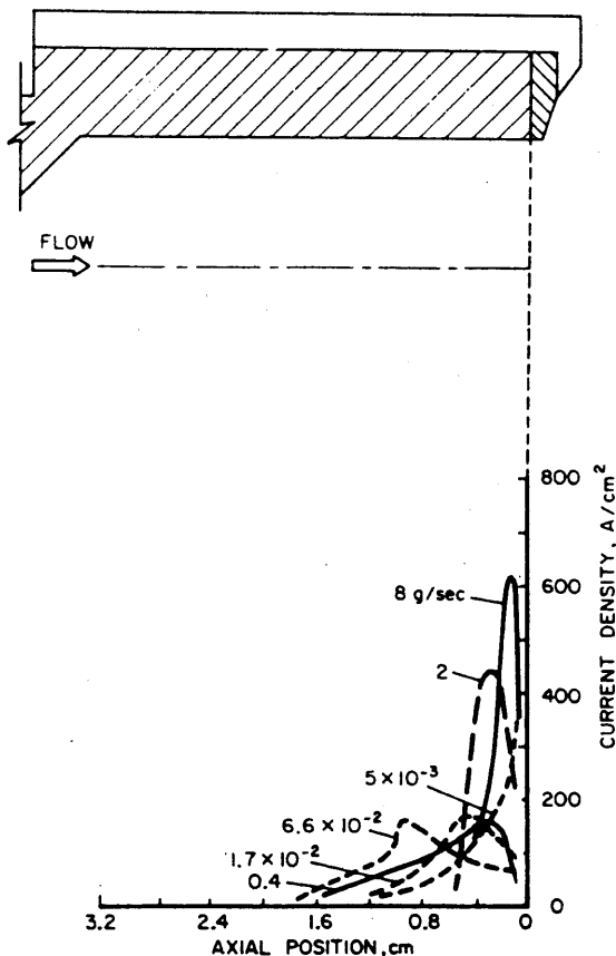
Fig. 4 Current density profiles, 0.9 kA.
