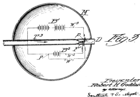
Figure 3: The the world’s first documented electrostatic thruster. Schematic of Goddard’s third variant of his 1917 invention as it appears in US patent #1,363,037 (granted in December 1920)[20]. The propellant is injected through the tube labeled T^3 ; charge is added to the flow from the cathode filament F^1 which is placed in the wake of the stream and whose anode is a metallic plate at location P . The filament is powered by the power supply B^2 . The whole is enclosed in a metallic sphere M , which is “kept at a very high potential” using the power supply B^1 . “The sign of the charge on M is the same as that of the ions in the jet thus causing their repulsion away from the device at high velocities proportional to the applied potential[20].”
