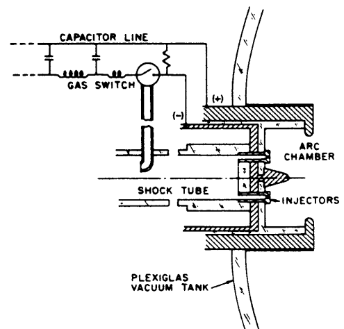
Fig. 1 Accelerator schematic.
