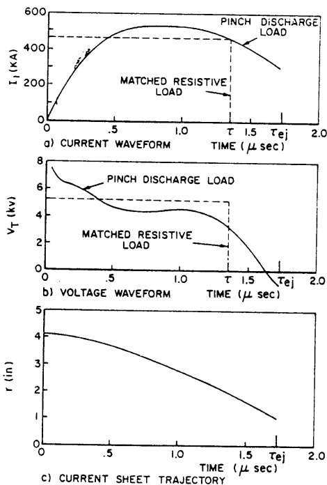
Fig. 3 Theoretical results: R_s = 0.002 \Omega , R_D = 0.0001 \Omega , r_0 = 0.117 \text{ m} , r_1 = 0.105 \text{ m} , h = 0.0508 \text{ m} , L_s = 3.00 \times 10^{-9} \text{ h} , \rho = 0.00022 \text{ kg/m}^3 , \tau = 2 n(LC)^{1/2} = 1.3 \times 10^{-6} \text{ sec} , Z_L = (L/C)^{1/2} = 0.00113 \Omega , V_0 = 10,500 \text{ v} .
