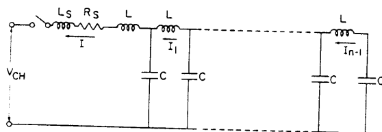
Fig. 2 Schematic of pulse line-accelerator system.
