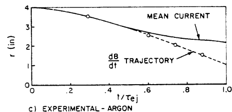
Fig. 14 Current trajectories: \rho = 0.00022 \text{ kg/m}^3 , V_0 = 10,500 \text{ v} , \tau = 1.7 \text{ } \mu\text{sec} , Z_L = 0.0113 \text{ } \Omega .
