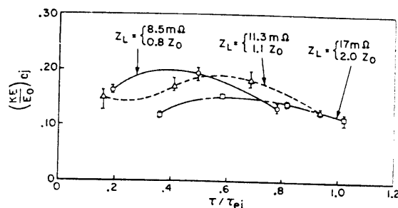
Fig. 11 Efficiency profiles: krypton (experimental).
