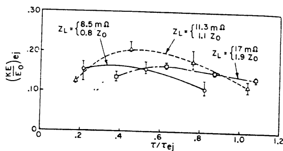
Fig. 10 Efficiency profiles: nitrogen (experimental).
