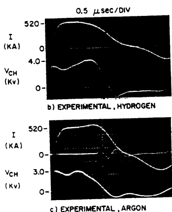
Fig. 13 Voltage and current waveforms: \rho = 0.00022 \text{ kg/m}^3 , V_0 = 10,500 \text{ v} , \tau = 1.7 \text{ } \mu\text{sec} , Z_L = 0.0113 \text{ } \Omega .
