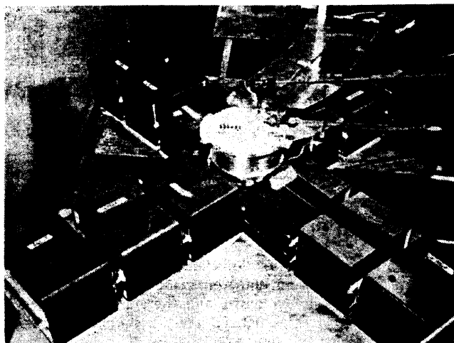
Fig. 7 Typical capacitor configuration.
