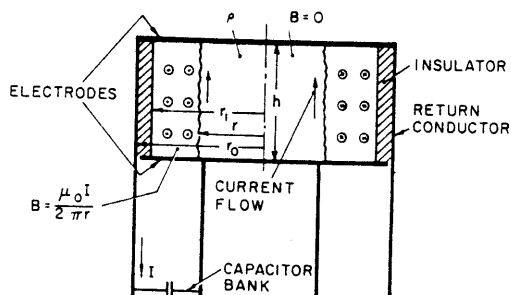
Fig. 1 Pinch discharge configuration.
