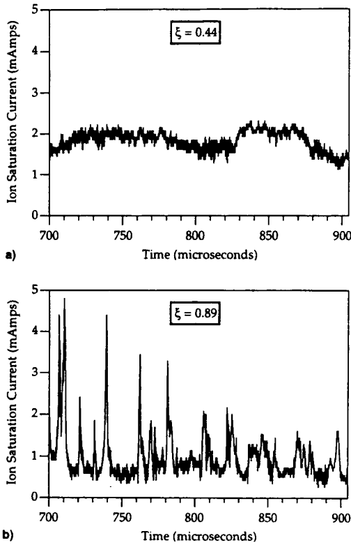
Fig. 9 Ion saturation current time histories for \xi = a) 0.44 and b) 0.89 with aluminum anode.
