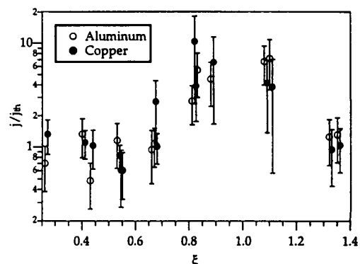
Fig. 8 Ratio of discharge to thermal current density.
