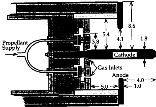
Fig. 1 MPD thruster (dimensions in cm).
