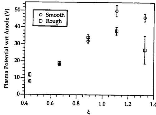
Fig. 11 Plasma potential a few millimeters from smooth and roughened aluminum anodes.
